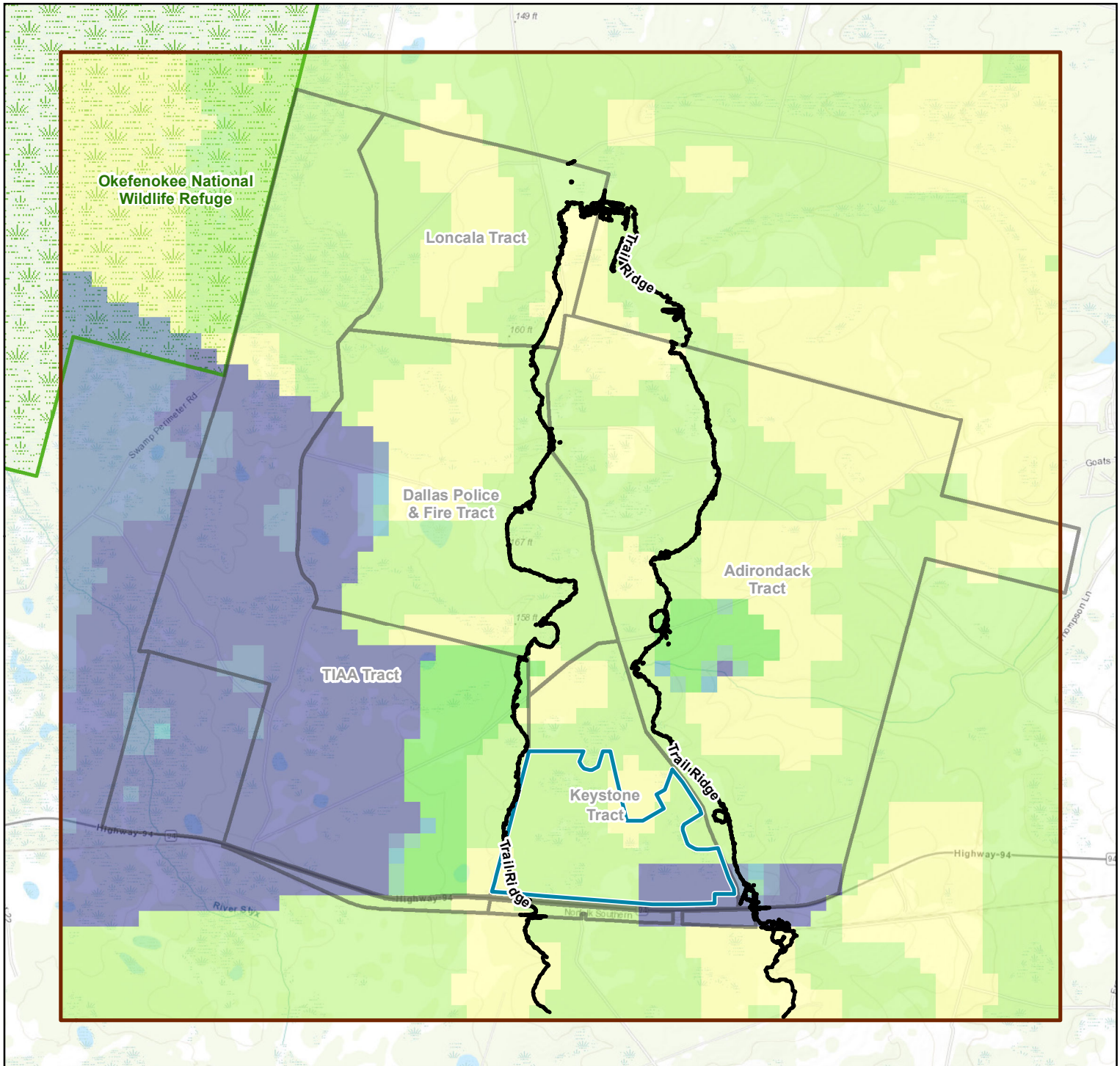
Figure 27 Calibrated Horizontal Hydraulic Conductivity in Consolidated Black Sands (HSU 2) Twin Pines Minerals, LLC St. George, Charlton County, Georgia
