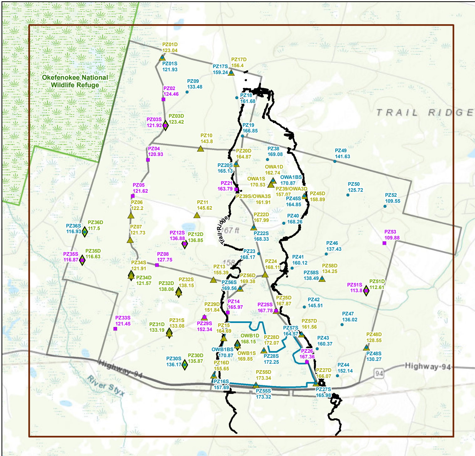
Figure 19 Average Well and Piezometer Groundwater Elevations January 2019 - October 2019 Twin Pines Minerals, LLC St. George, Charlton County, Georgia
