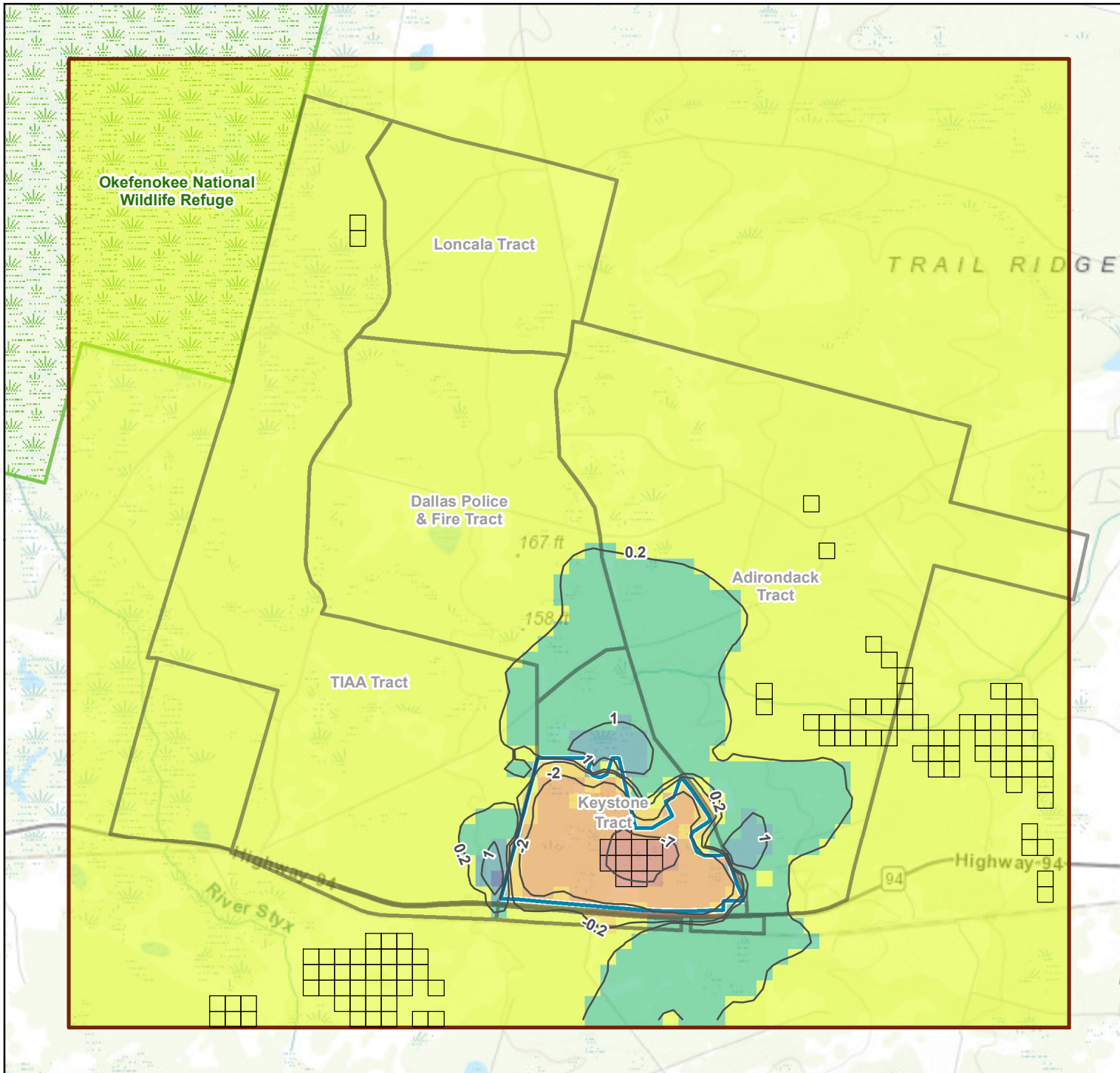
Figure 42 Water Table Difference 12.5% Bentonite Soil Amendment Twin Pines Minerals, LLC St. George, Charlton County, Georgia
