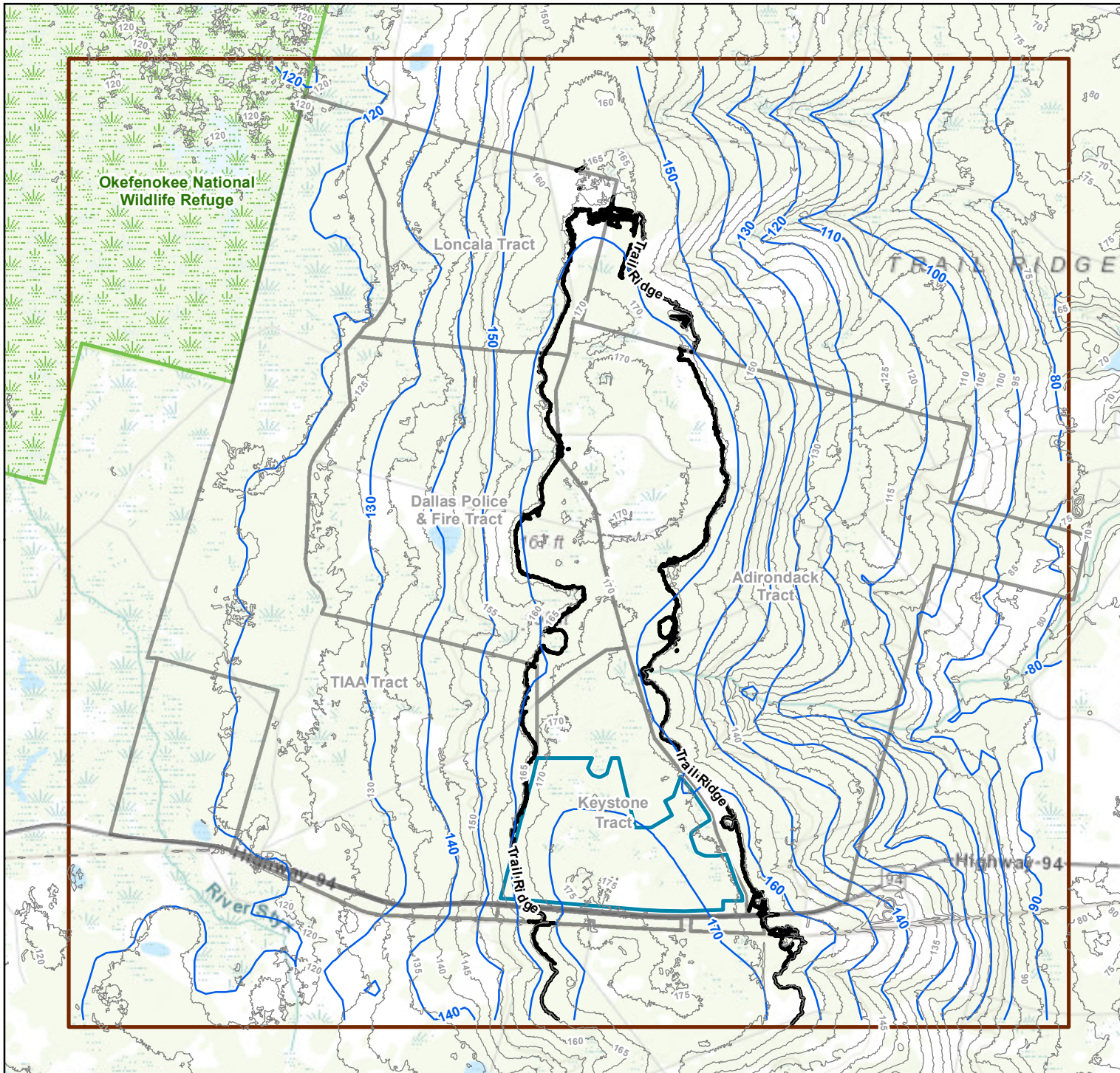
Figure 35 Simulated Water Level Contours for Post-Mining Conditions with No Bentonite Twin Pines Minerals, LLC St. George, Charlton County, Georgia
