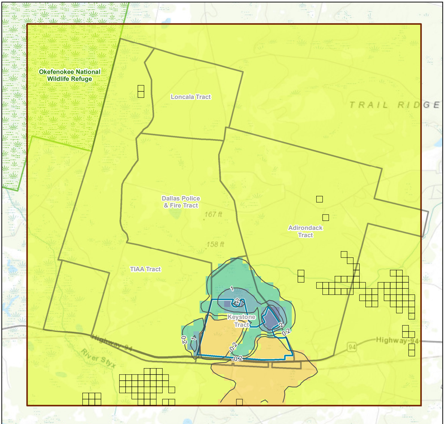
Figure 39 Water Table Difference No Bentonite Soil Amendment Twin Pines Minerals, LLC St. George, Charlton County, Georgia
