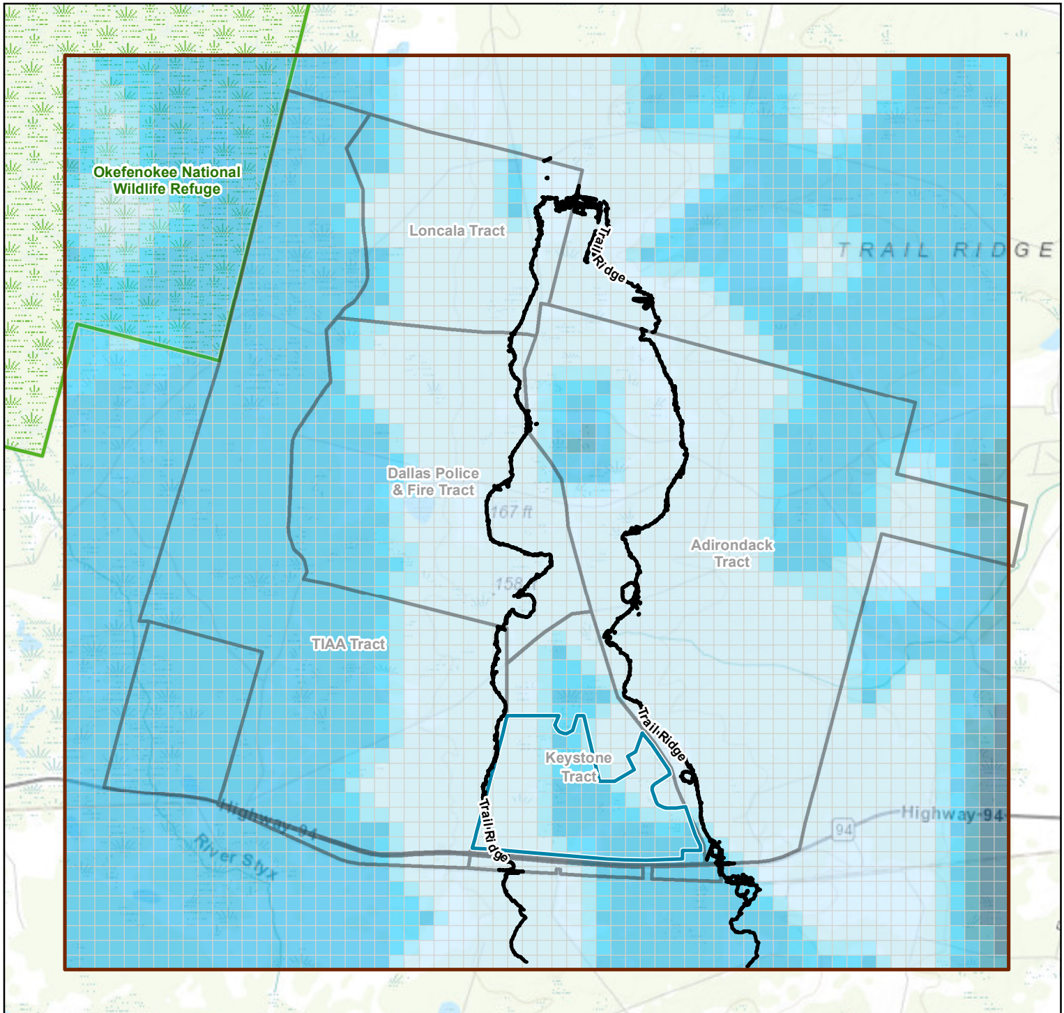
Figure 29 Calibrated Horizontal Hydraulic Conductivity in Sandy Clay Unit (HSU 4) Twin Pines Minerals, LLC St. George, Charlton County, Georgia
