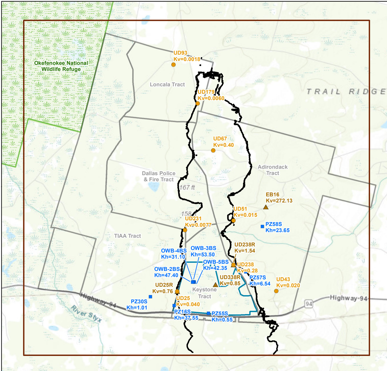
Figure 15 Unconsolidated & Semiconsolidated Sand (Hydrostratigraphic Unit 1) Hydraulic Conductivity Twin Pines Minerals, LLC St. George, Charlton County, Georgia
