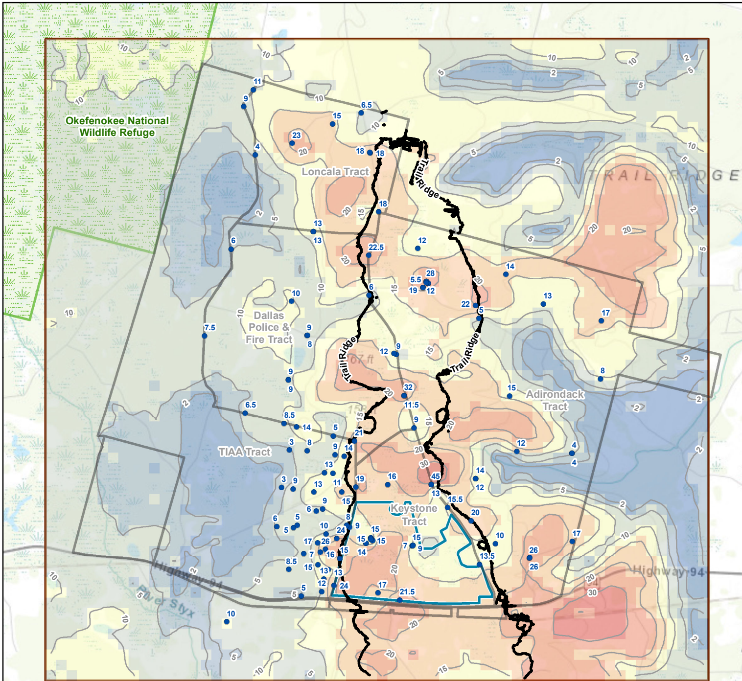
Figure 7 Unconsolidated & Semiconsolidated Sand (Hydrostratigraphic Unit 1) Thickness
